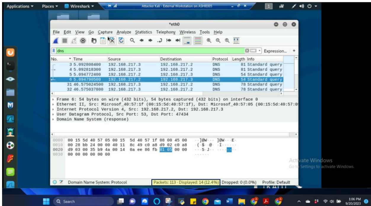
Figure 4 Screenshot of Wireshark with “DNS” filter in Attacker Linux for Task A.4
