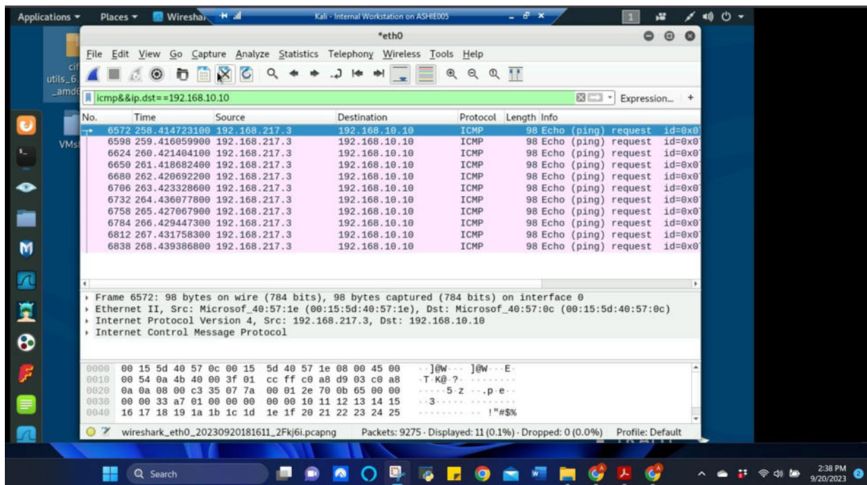
Figure 8 Screenshot of Wireshark on Internal Kali sniffing traffic between External Kali and Ubuntu VM. This shows the “ICMP” and “ip destination of ubuntu” filter being used for Task B.1b
