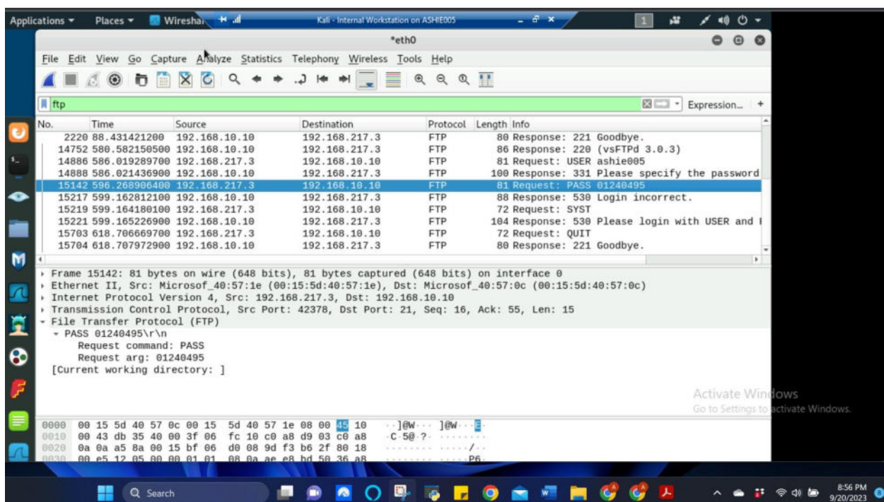
Figure 12 Screenshot of Wireshark from Internal Kali showing the “FTP” traffic by using the “FTP” filter for Task B.2c
