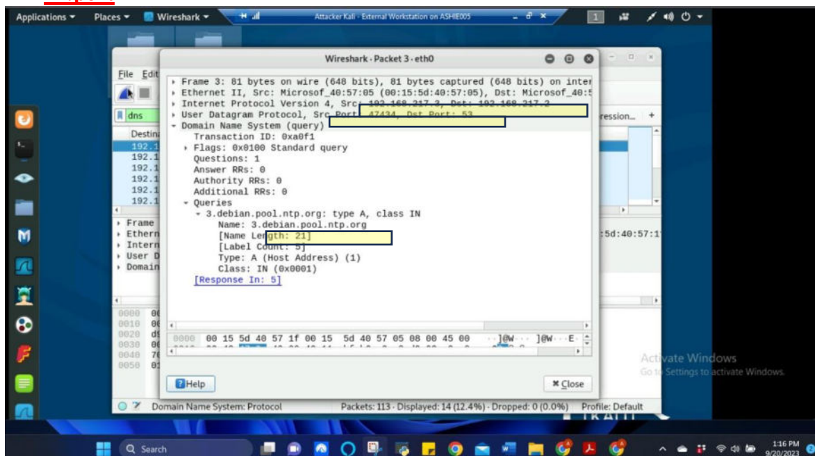
Figure 5 Screenshot of DNS query packet from Packet 3 in Wireshark on Attacker Linux for Task A.5
