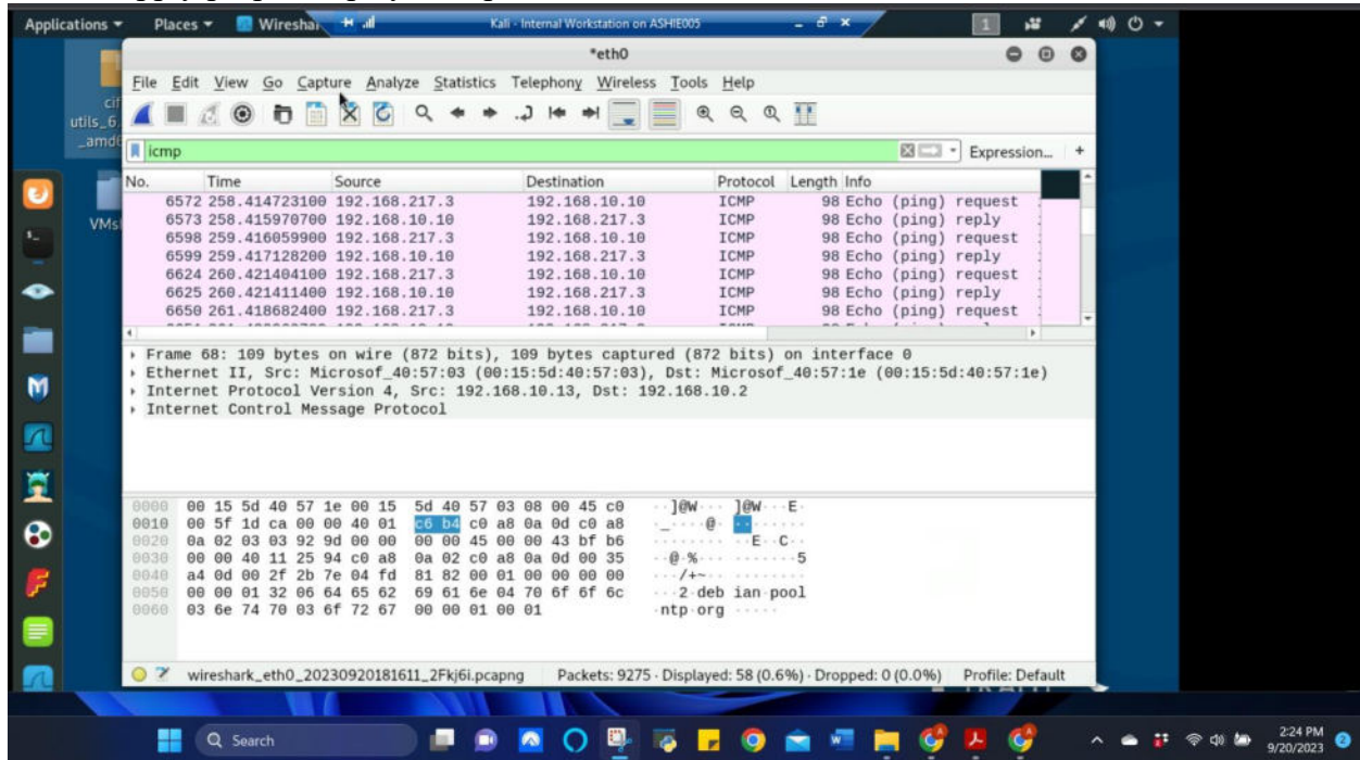
Figure 7 Screenshot of Wireshark on Internal Kali sniffing traffic between External Kali and Ubuntu VM. This shows the “ICMP” filter being used for Task B.1a
