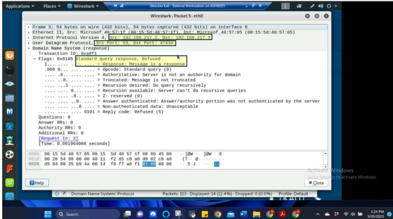
Figure 6 Screenshot of corresponding DNS response from Packet 5 in Wireshark on Attacker Linux for Task A.6
