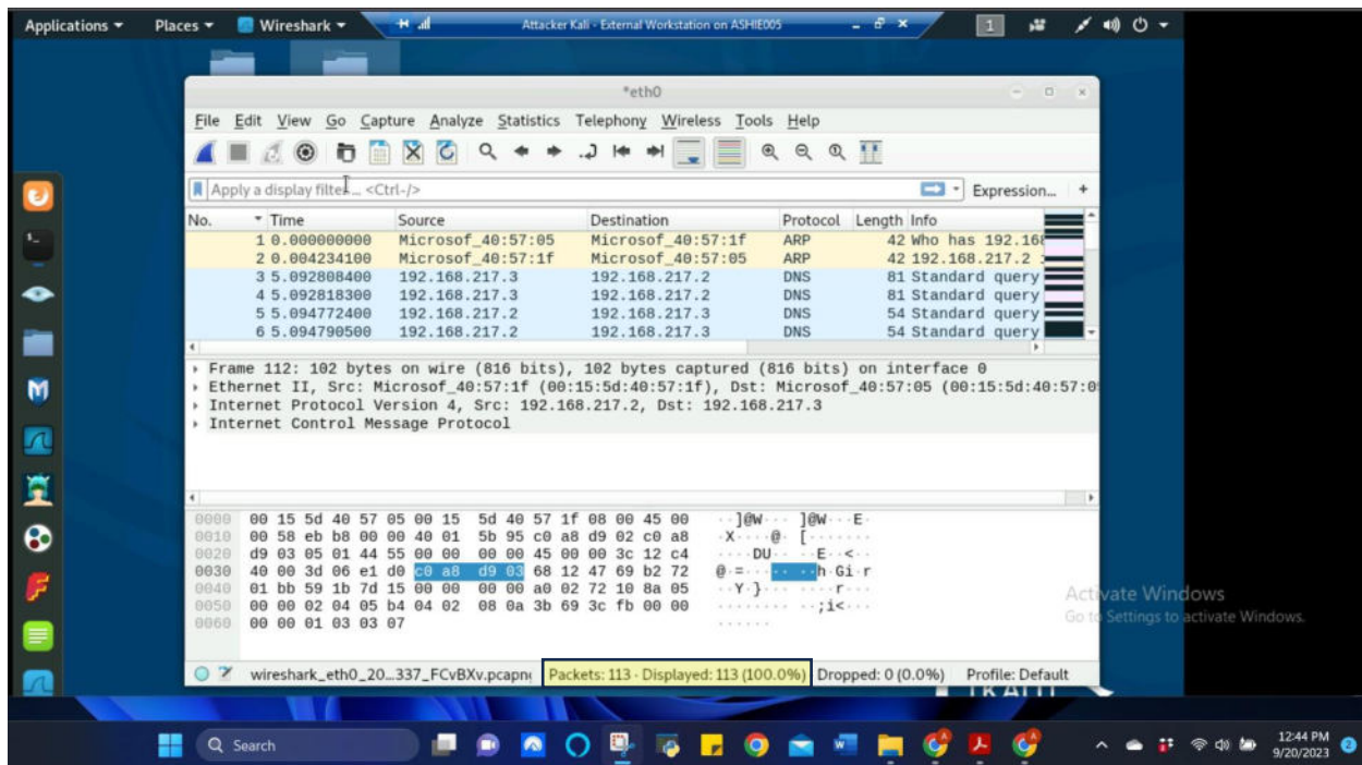
Figure 1 Screenshot of Wireshark in Attacker Linux for Task A.1
