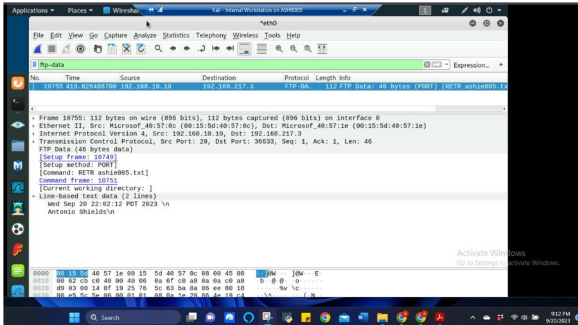
Figure 15 Screenshot of Wireshark from Internal Kali showing the “FTP-data” traffic by using the “FTP-data” filter for Task EC-1
