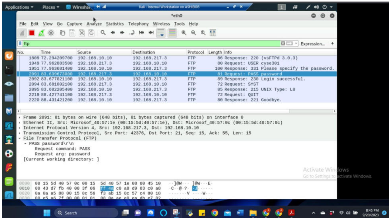
Figure 10 Screenshot of Wireshark from Internal Kali showing the “FTP” traffic by using the “FTP” filter for Task B.2b
