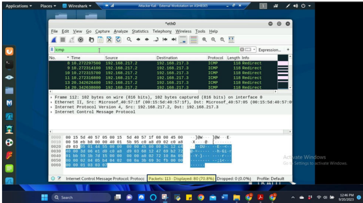
Figure 2 Screenshot of Wireshark with “ICMP” filter in Attacker Linux for Task A.2
