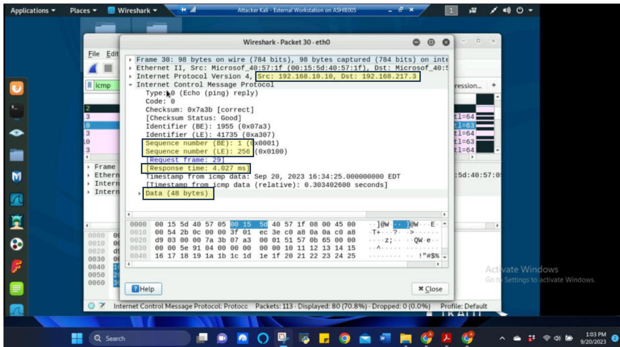
Figure 3 Screenshot of Echo reply message from Packet 30 in Wireshark on Attacker Linux for Task A.3
