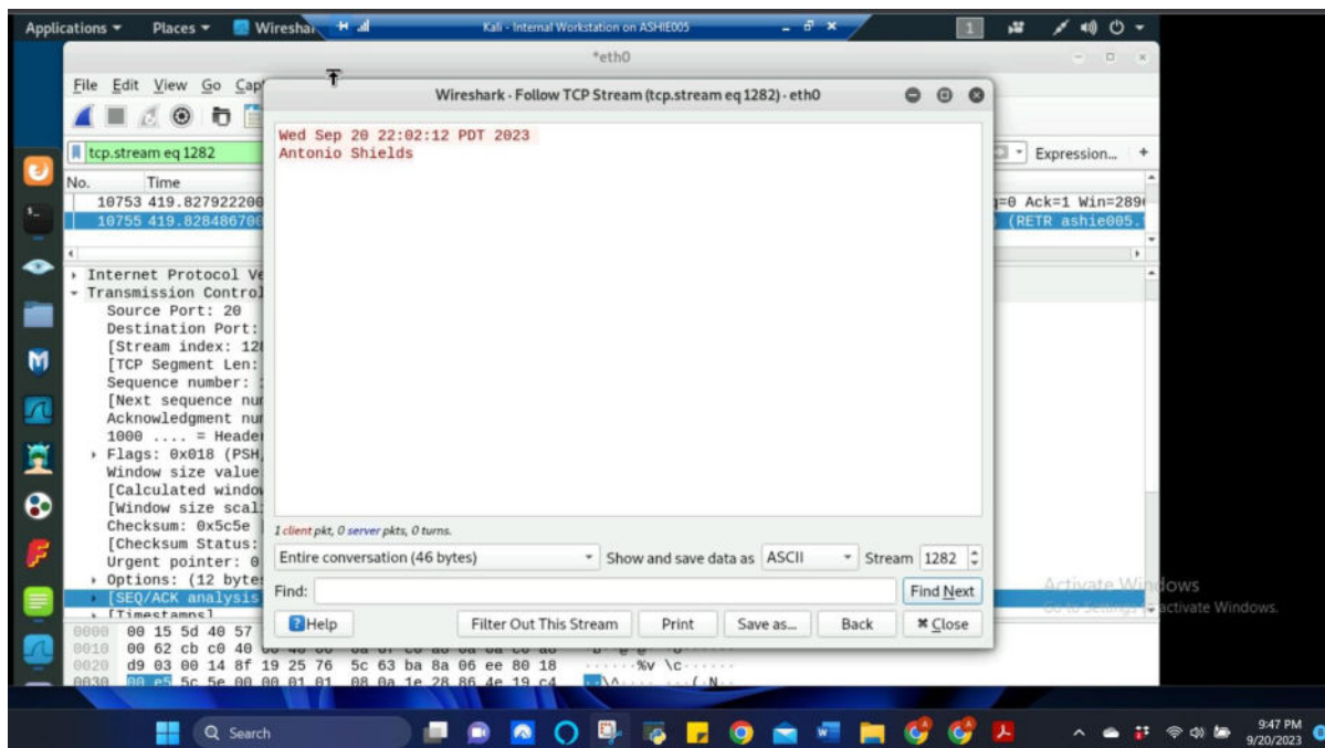
Figure 16 Screenshot of Wireshark from Internal Kali showing the TCP stream of the FTP-data packet and the contents of the file Task EC-2
