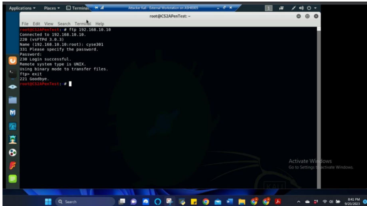
Figure 9 Screenshot of accessing the Ubuntu FTP Server using External Kali. This shows the ftp command in the External Kali terminal to access the FTP server in Ubuntu for Task B.2a
