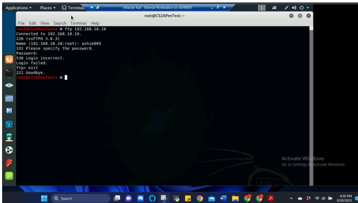
Figure 11 Screenshot of accessing the Ubuntu FTP Server again using External Kali. This shows the ftp command in the External Kali terminal to access the FTP server in Ubuntu for Task B.2c
