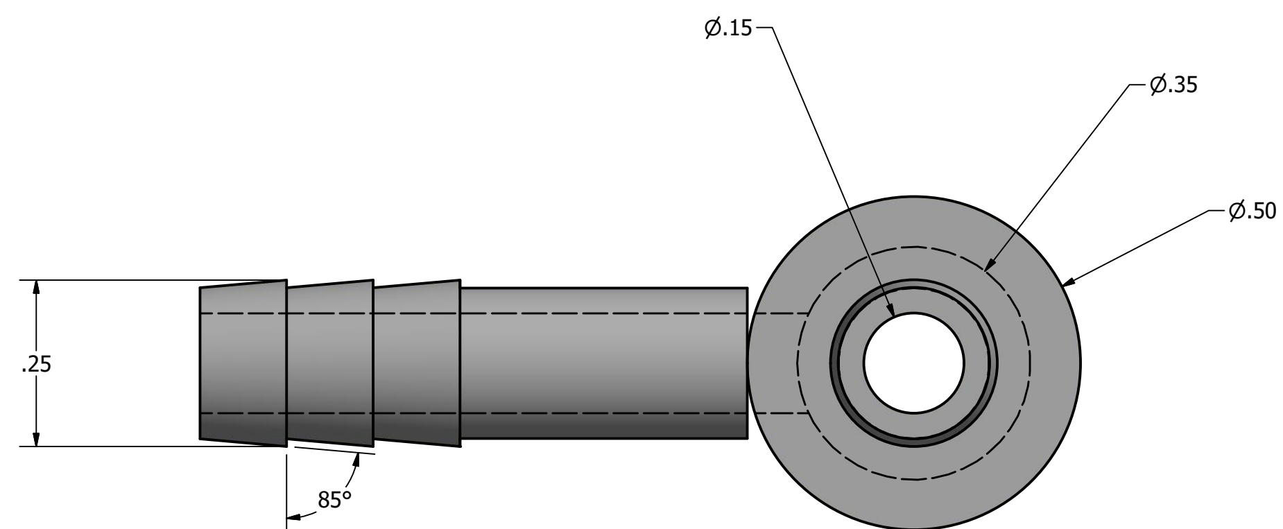
Front View
