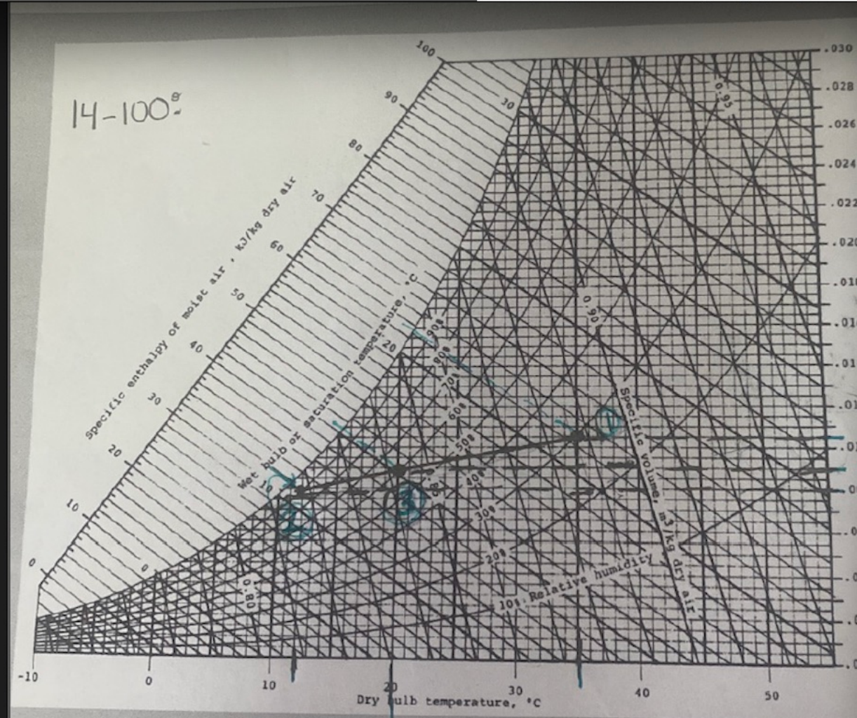
FIGURE A-31 Psychrometric chart at 1 atm total pressure.
